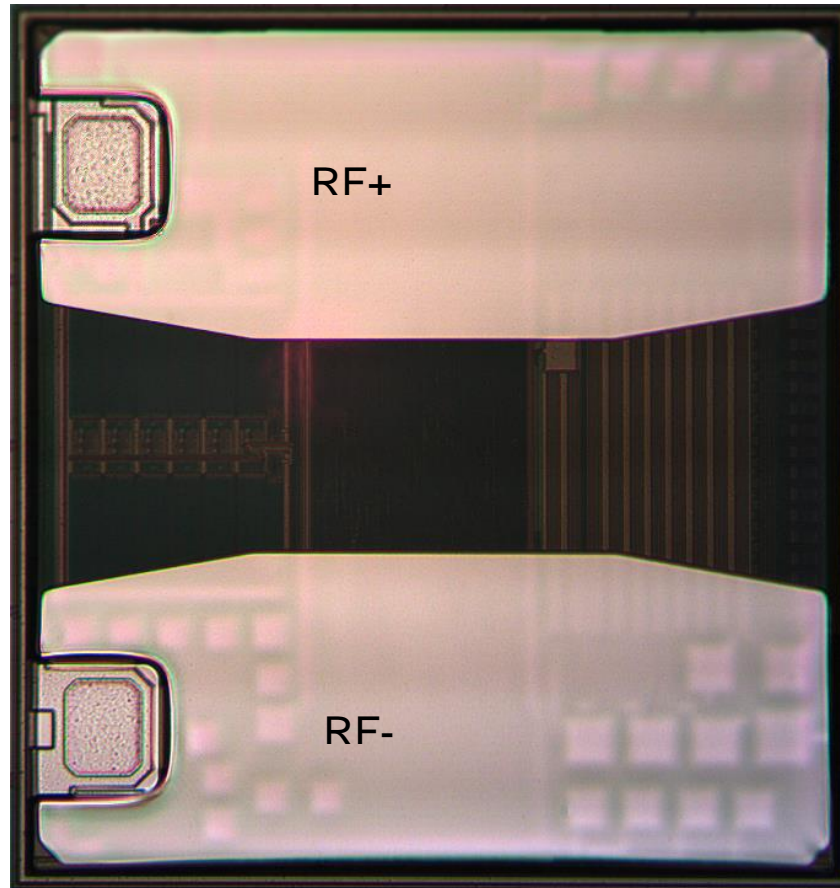
Figure 2-2 Monza R6-P Tag Chip Die Orientation
